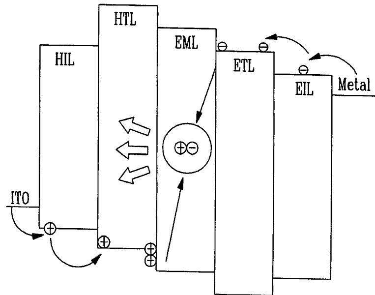
FIG. 2 RELATED ART
