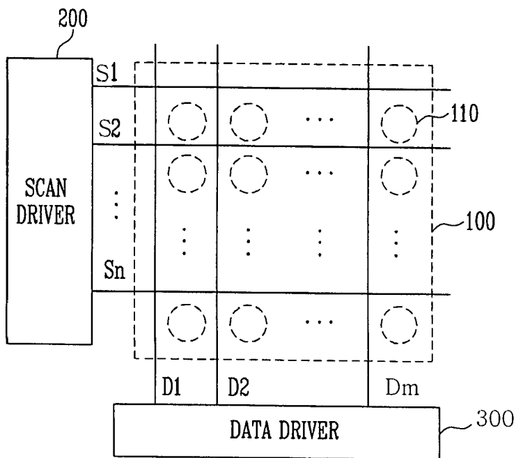
FIG. 3 RELATED ART
