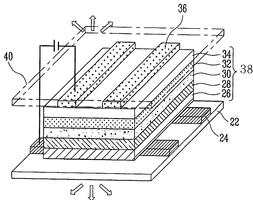
FIG. 2 RELATED ART
